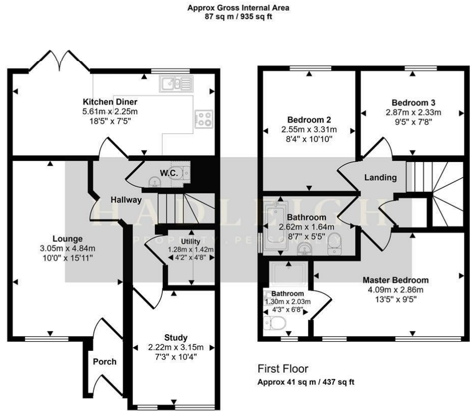
Ground Floor Approx 46 sq m / 498 sq ft
